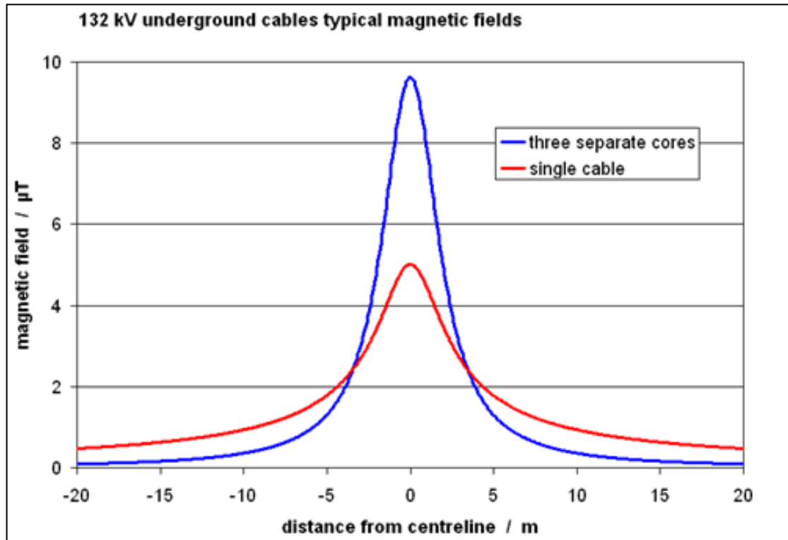
Figure 5 Typical magnetic fields associated with 132kV underground cable
